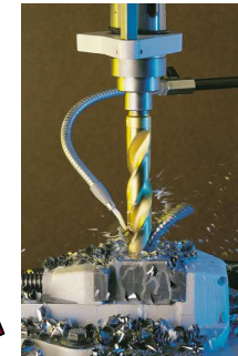
Loch bohren
